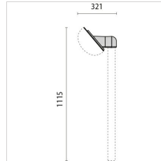
000800 Angled bracket for 42 mm post Black
